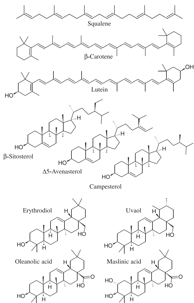
Fig. 1. Chemical structures of squalene, carotenoids, sterols, triterpenic dialcohols, and triterpenic acids in virgin olive oil.
